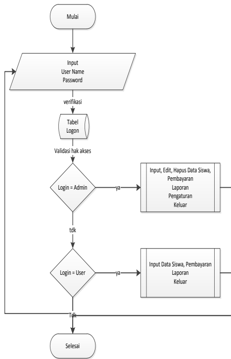
Gambar 3. Flowchart Login
