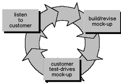
Gambar 1. Prototyping Model
