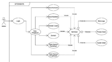
Gambar 6. Usecase Admin
